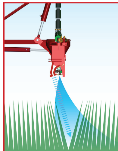
No wind, AirFlowPlus in neutral position
