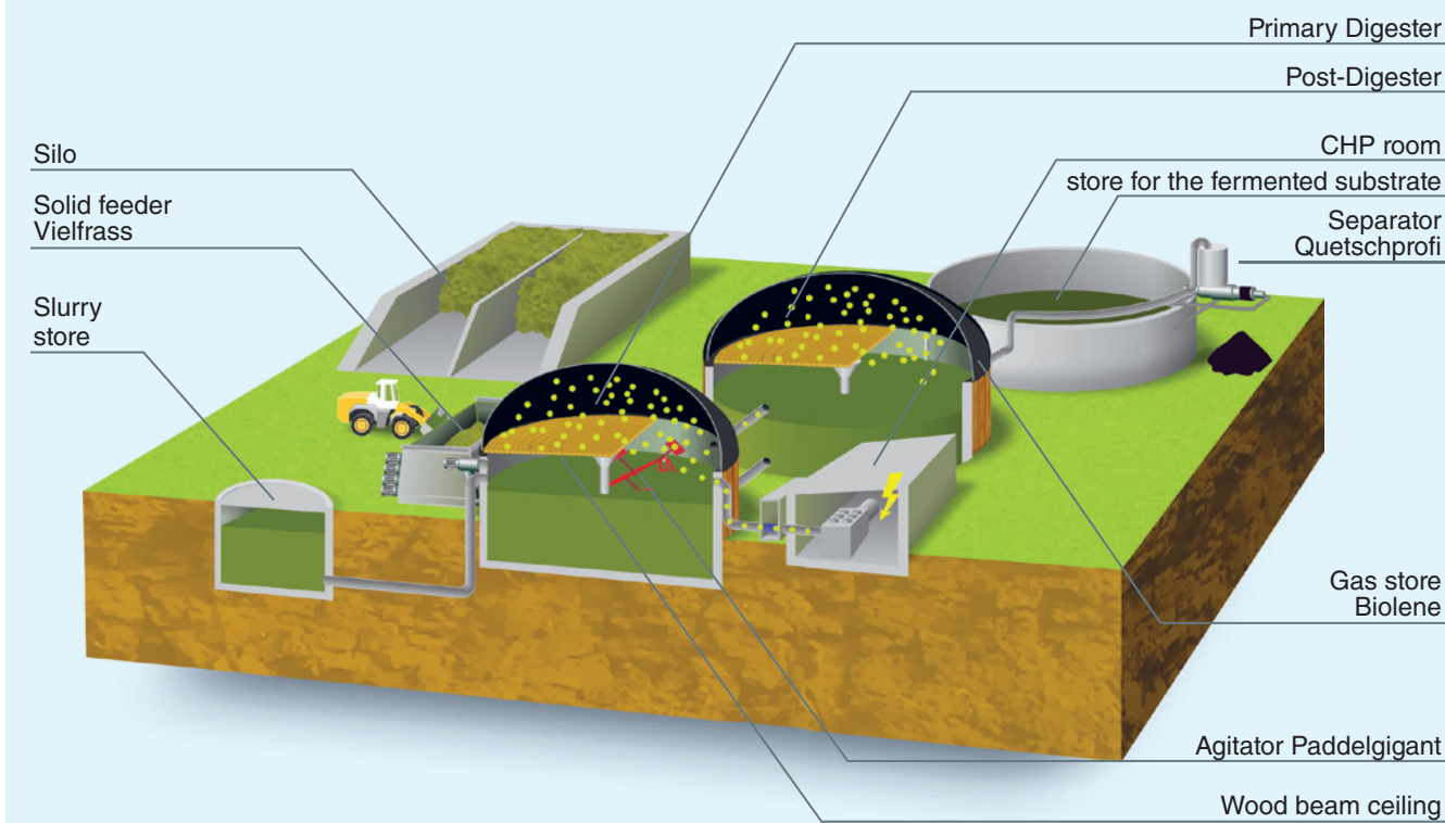
Functional diagram of a biogas plant made by agriKomp
